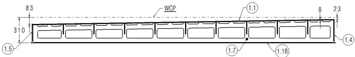
Figure 8: Typical sectional view showing longitudinal contour profile
