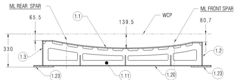
Figure 3: Typical sectional view showing transverse contour profile
