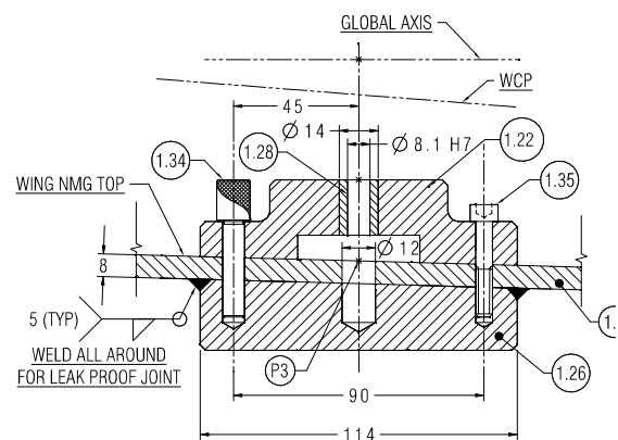
Sectional Details (all dimensions are in 'mm')
