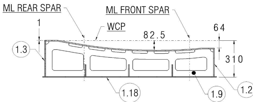
Figure 9: Typical sectional view showing transverse contour profile
