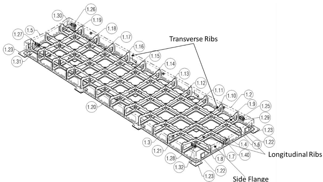
Figure 5: Wing bottom skin I/B LH tool backup structure (longitudinal, transverse ribs and side flanges)
