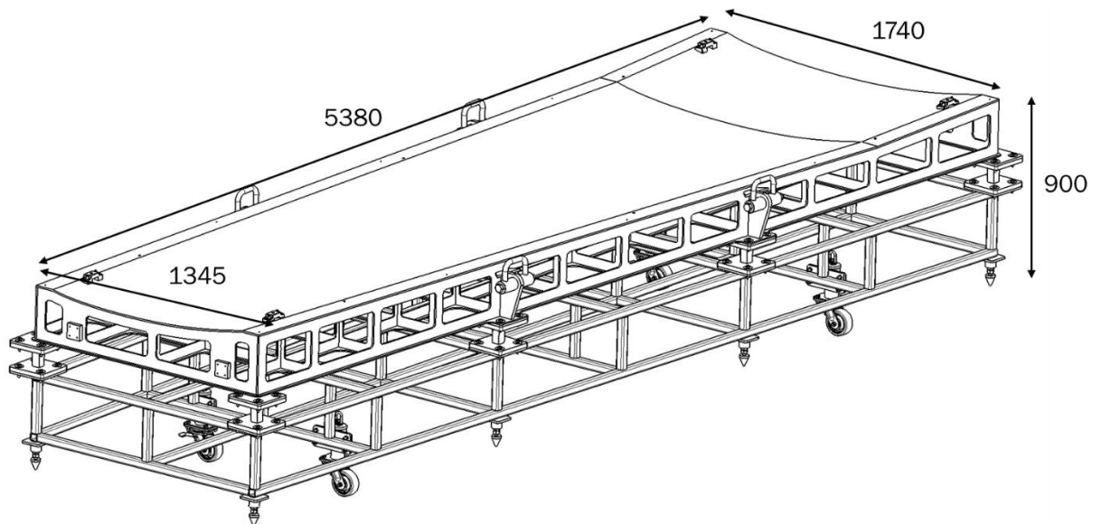
Figure 1: Wing bottom skin I/B LH tool including backup structure and support structure
